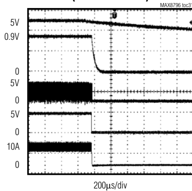
BIAS SUPPLY REMOVAL (UVLO RESPONSE)
