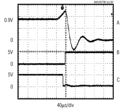
OUTPUT OVERVOLTAGE WAVEFORM
