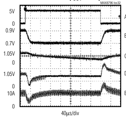
POWER MONITOR - VID TRANSITION RESPONSE ( I_{OUT} = 10\text{A} )
