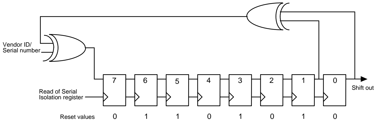
Figure 3. Checksum LFSR
