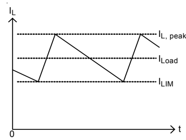
Figure 2. “valley” Current-Limit
