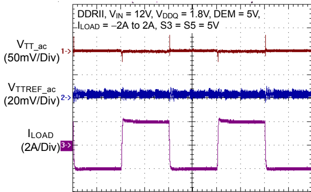
Time (500µs/Div)
