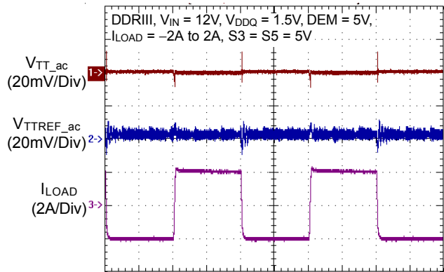
Time (500µs/Div)
