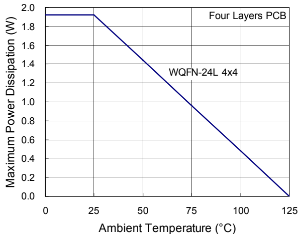
Figure 5. Derating Curves for RT8207 Packages
