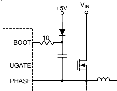
Figure 3. Reducing the UGATE Rise Time
