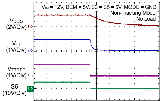
Time (2ms/Div)
