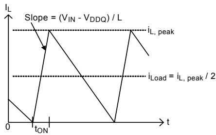
Figure 1. Boundary condition of CCM/DCM
