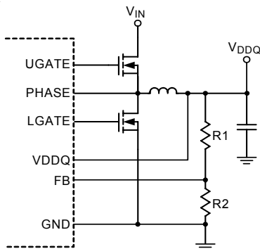
Figure 4. Setting VDDQ with a Resistor-Divider
