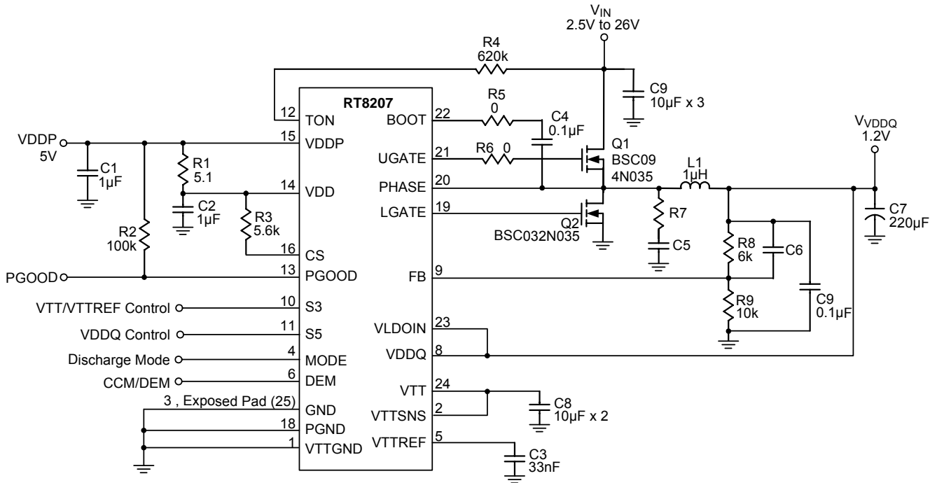
Figure A. Adjustable Voltage Regulator
