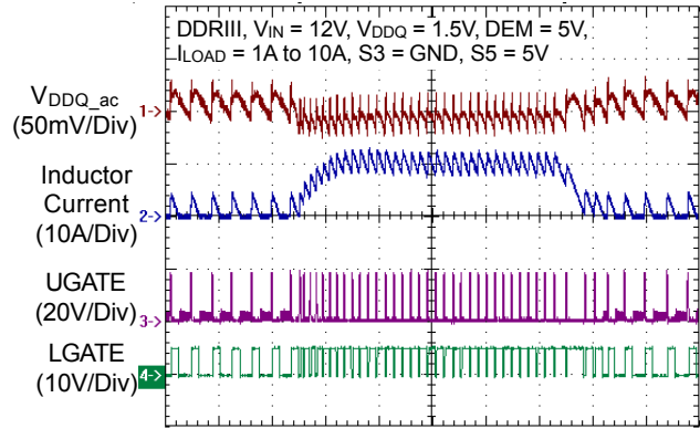
Time (20µs/Div)
