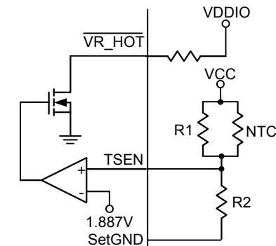
Figure 22. VR_HOT Circuit
