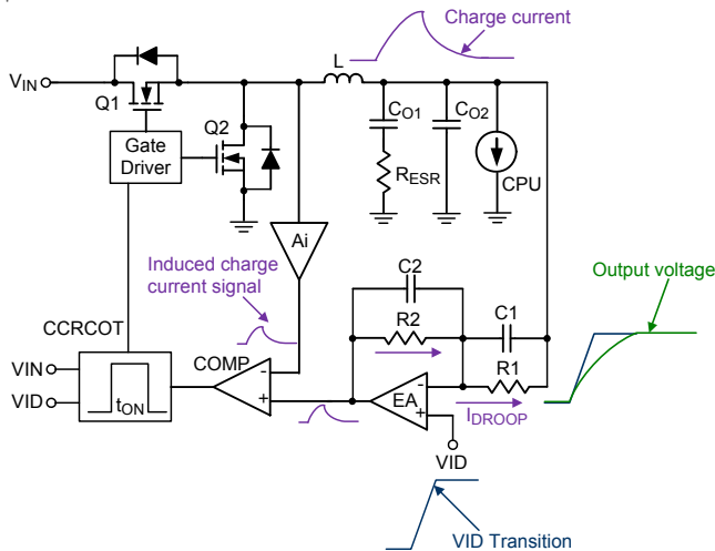
Figure 15. Droop Effect in VID Transition
