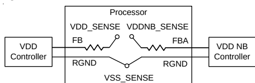
Figure 5. Differential Remote Voltage Sense Connection
