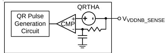
Figure 21. VDDNB Controller : Quick Response Triggering Circuit
