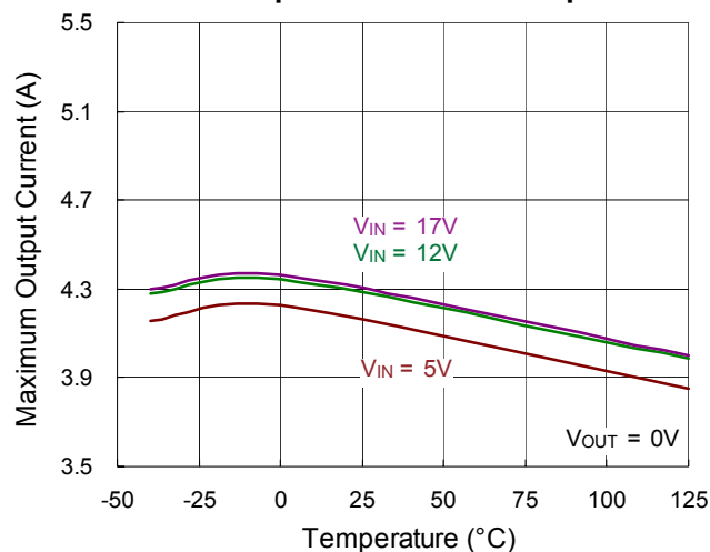
Maximum Output Current vs. Temperature
