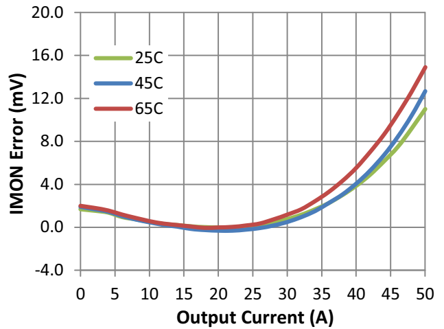
Figure 19. I_{MON} Accuracy vs. Temperature
