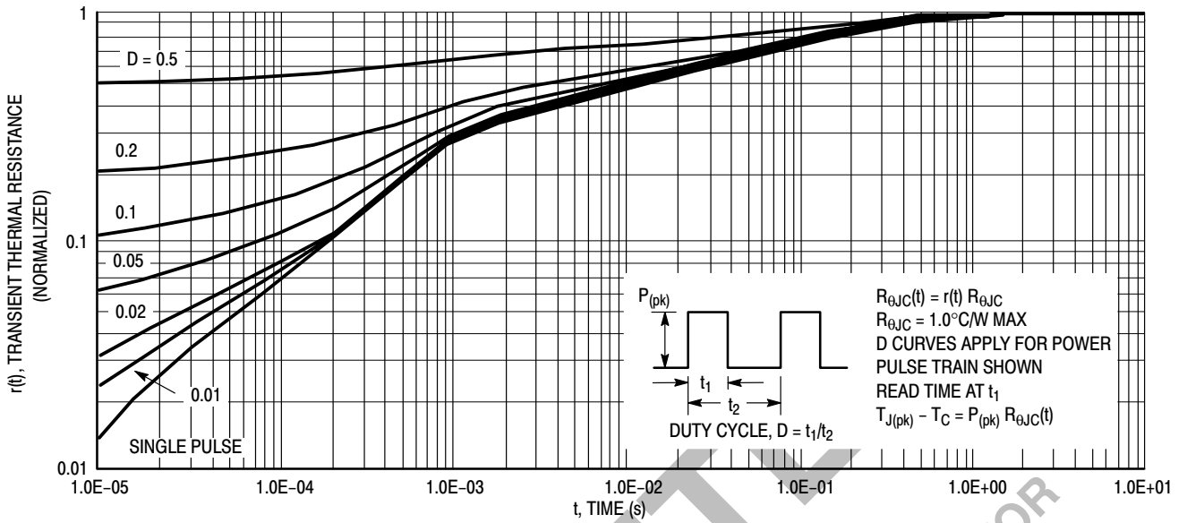
Figure 14. Thermal Response
