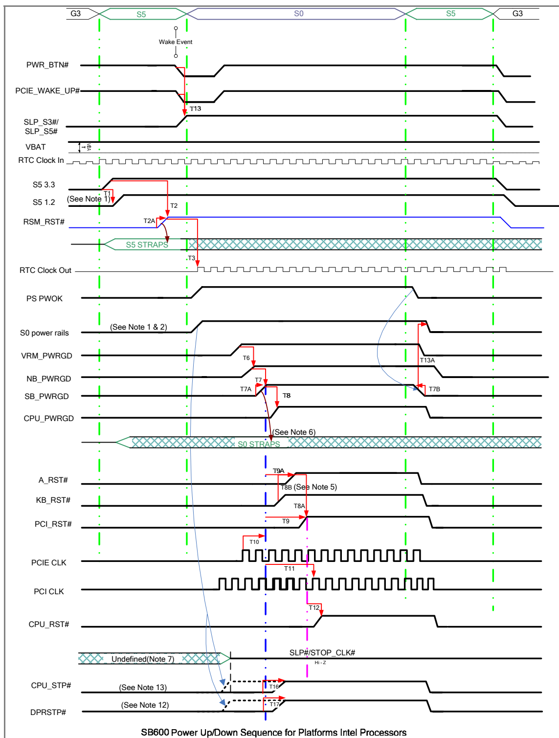
Figure 4-1: SB600 Power Up/Down Sequence for Platforms with Intel Processors
