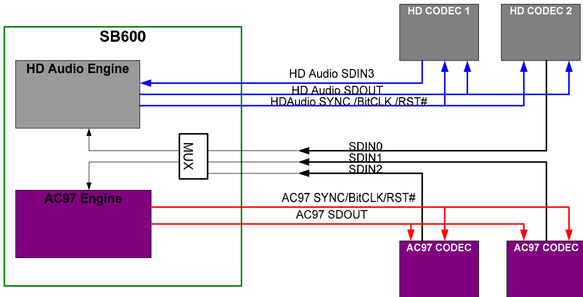
Figure 5-12: HD Audio and AC '97 Codec Connections for Mixed Configurations
