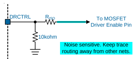
Figure 5. DRCTRL Connection
