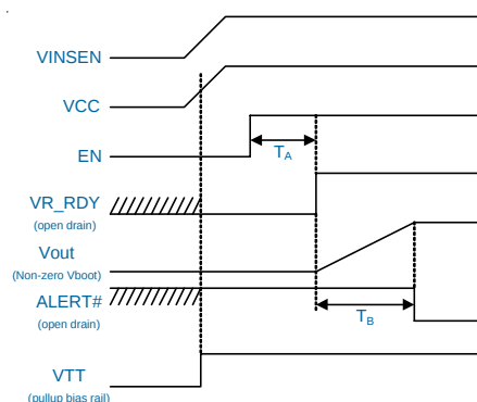
Figure 2. Start up Sequence and Enable Timing with Non-zero Vboot
