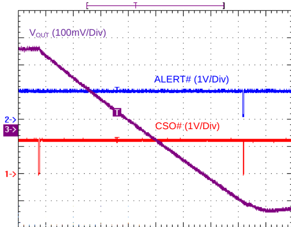
VccGT SetVID_Decay
