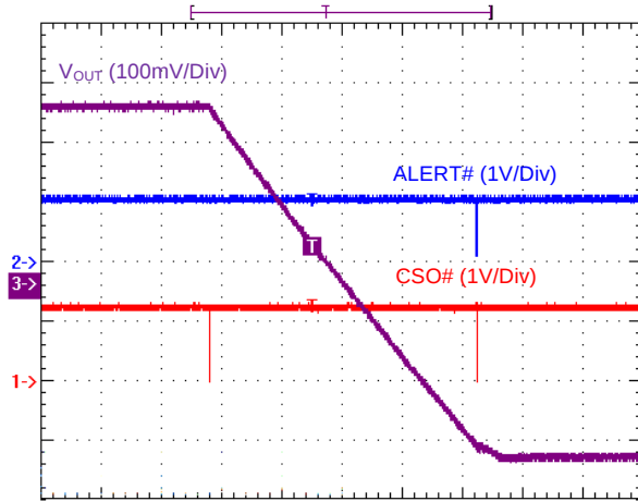
Vcore SetVID_Decay
