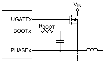
Figure 6. Increasing the UGATEx Rise Time
