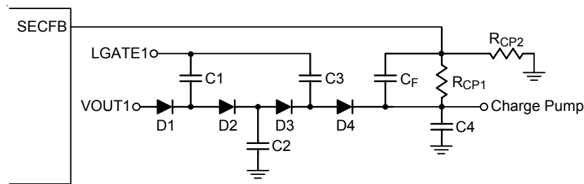
Figure 5. Charge pump circuit connected to SECFB
