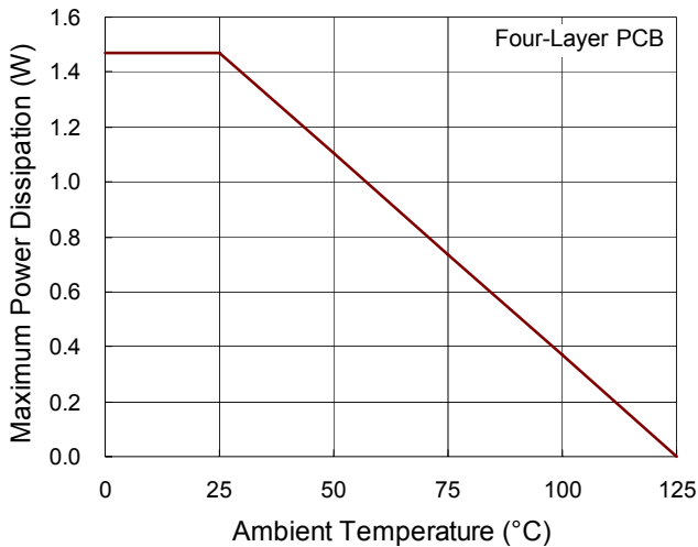
Figure 8. Derating Curve for the RT8239A/B/C Package
