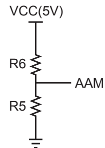
Figure 4— AAM Network
