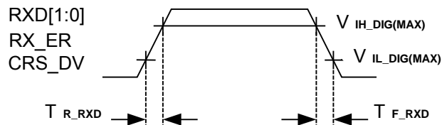
Figure 6: RMI Rise and Fall Times
