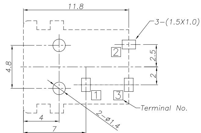
Recommended PCB Layout (Printed-sided View)
