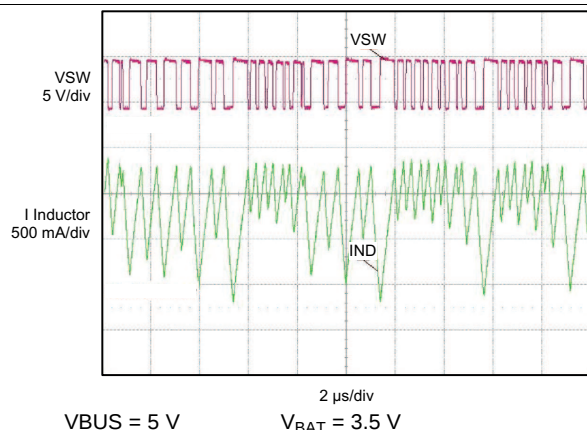
Figure 1. Cycle by Cycle Current Limiting In Charge Mode Overload Operation
