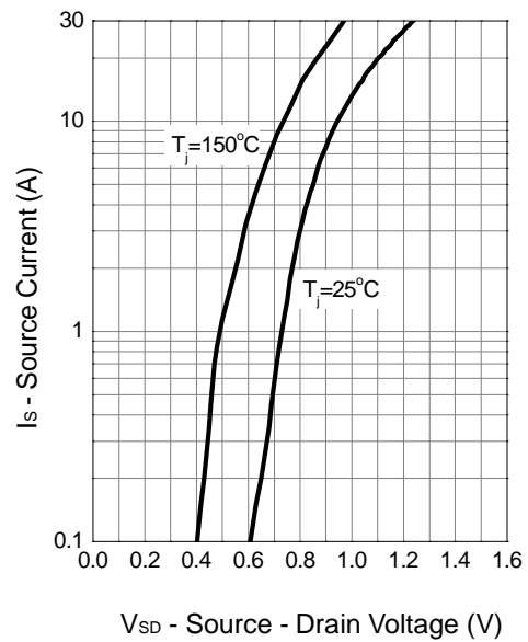
Source-Drain Diode Forward
