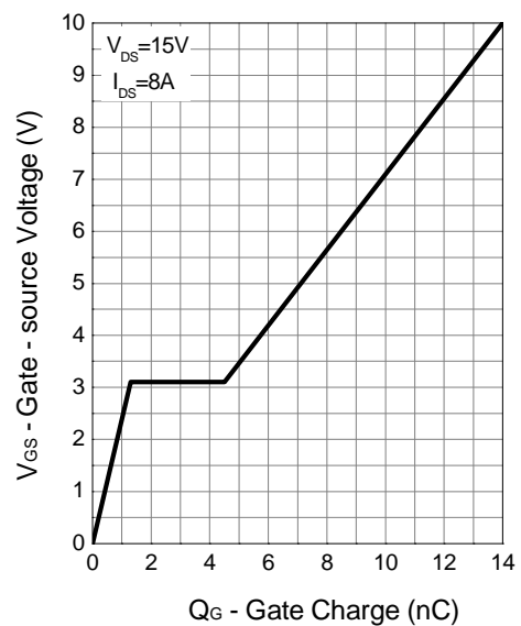
Gate Charge
