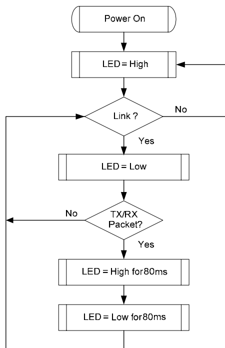
Figure 5. LINK/ACT LED
