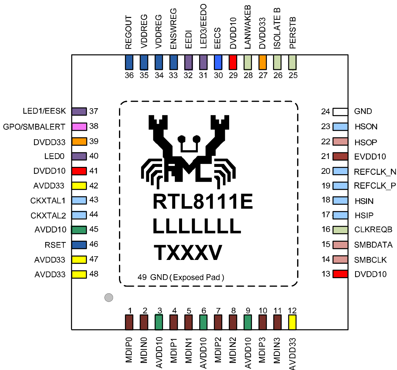
Figure 1. Pin Assignments
