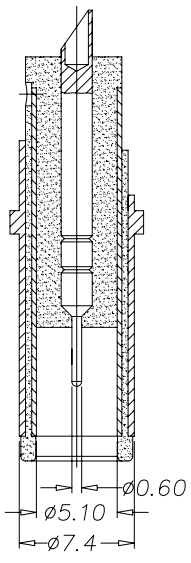
MATING PLUG: OD \phi 7.4 ; ID \phi 0.6 Tolerance: \pm 0.05
