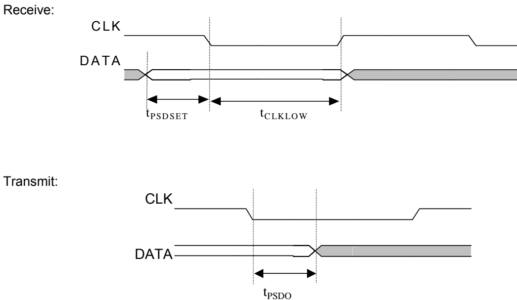
Figure 9-13. PS/2 Receive/Transmit Timing
